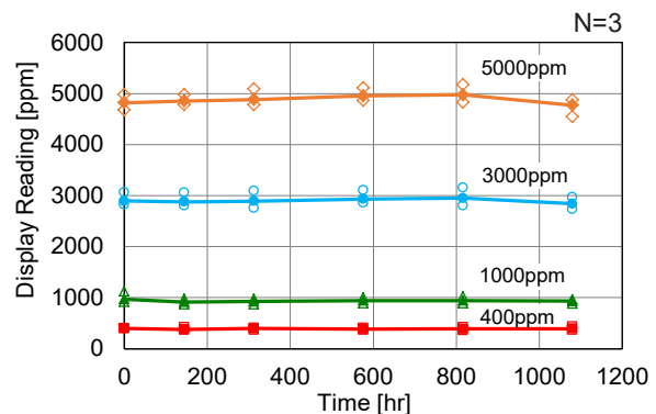
Fig. 7 - Durability to high temperature and high humidity
