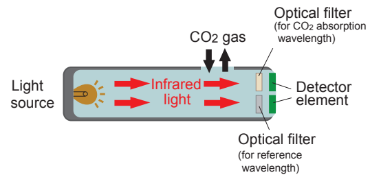
Fig. 2 - Basic structure of CDM7162 optics
