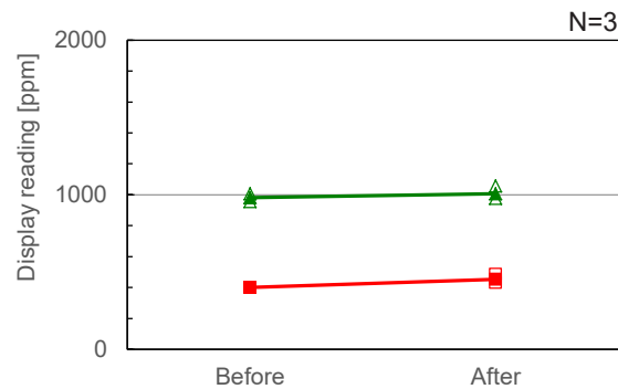
Fig. 9-1 - Corrosion test against H 2 S
