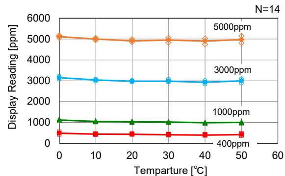
Fig. 6 - Temperature dependency
