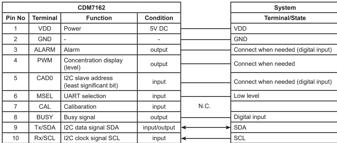
Fig. 13 - I2C connections
