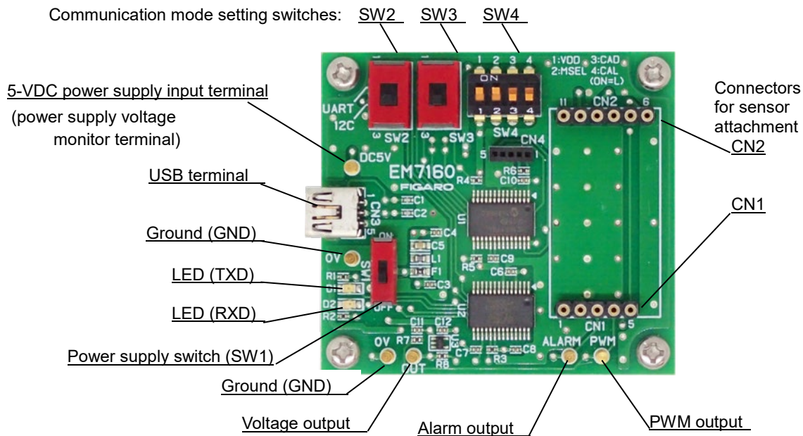
Figure 1 - Parts
