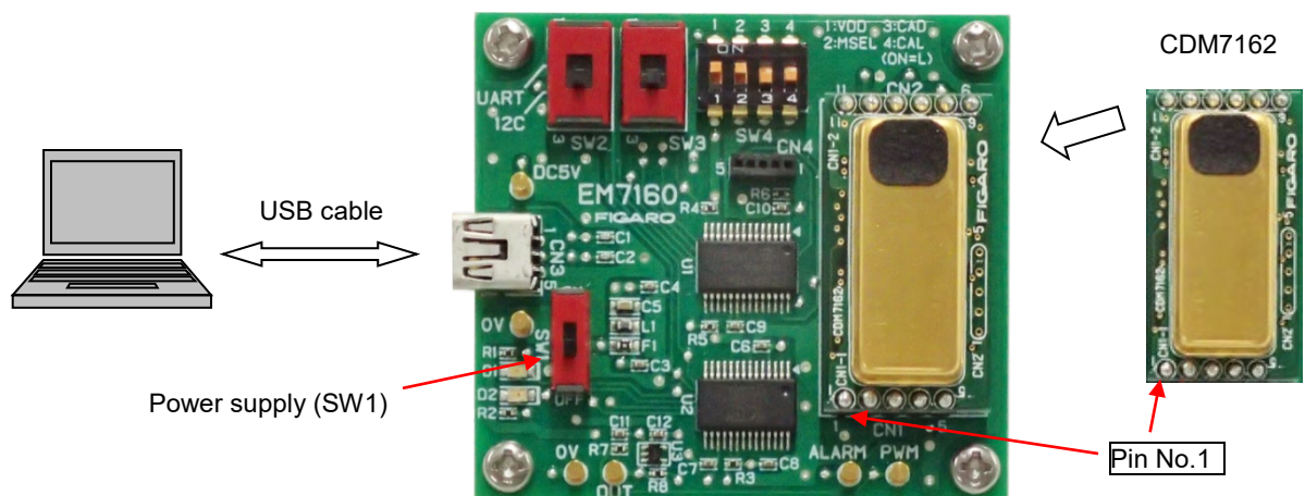
Figure 4 - Attachment of CDM7162
