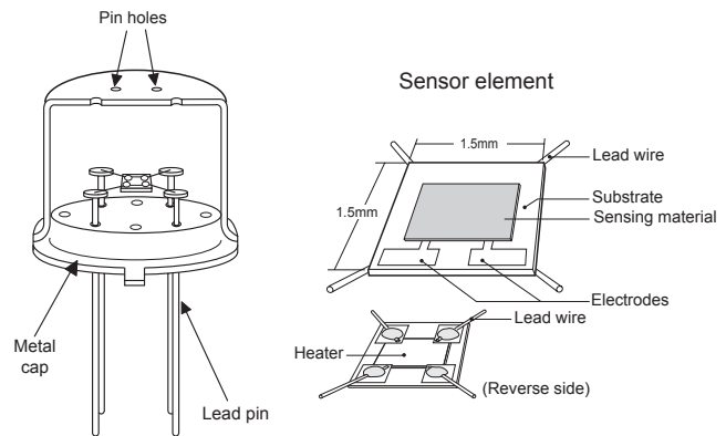
Fig. 1 - Sensor structure
