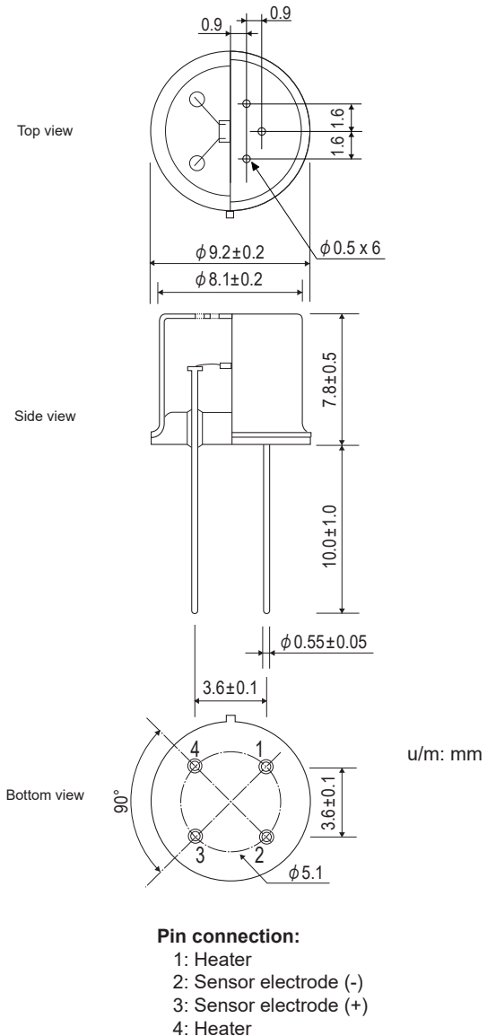
Fig. 3 - Sensor dimensions
