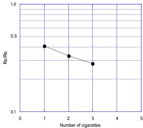
Fig. 5 - Sensitivity to cigarette smoke ( R_s/R_o )
