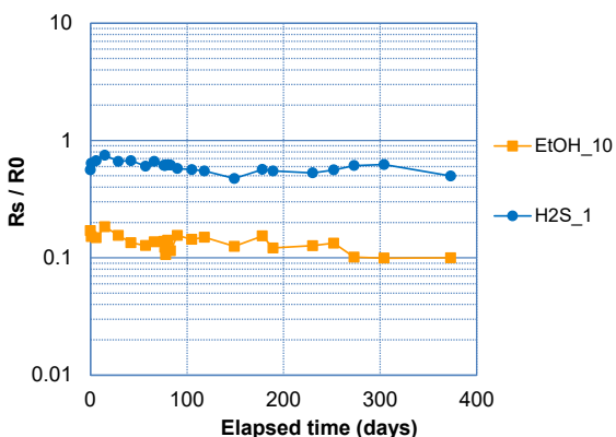
Fig. 16-1 - Long term stability (continuous energizing) in various gases
