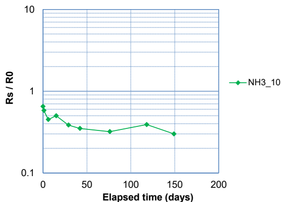
Fig. 16-2 - Long term stability (continuous energizing) in various gases
