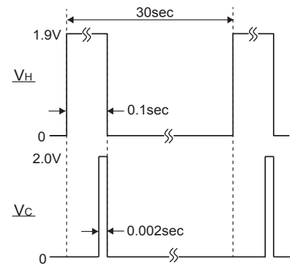
Timing chart
